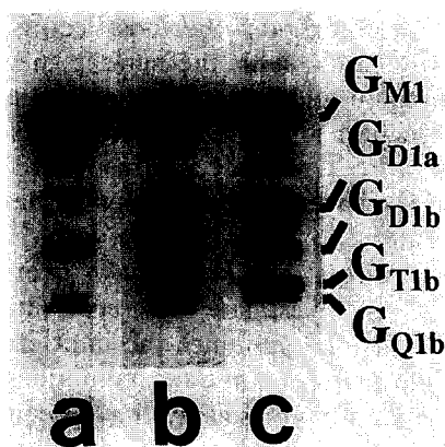
Fig. 5. Detection of gangliotetraose-type gangliosides by combined neuraminidase and cholera toxin-immunostaining assay. 25 ng (lanes a and b, each) and 10 \mu g of human brain gangliosides (lane c) were chromatographed as described in Fig. 3. Lane a: combined immunostain with cholera toxin and anti-cholera toxin antibody; lane b: V. cholerae neuraminidase treatment prior to cholera toxin detection; lane c: resorcinol stain [134]. Structures of gangliotetraose-type gangliosides are listed in Table 2.
