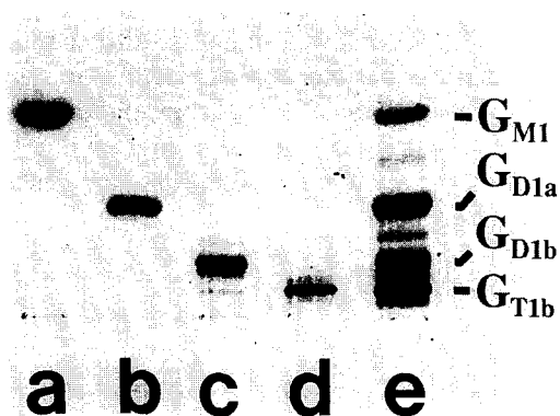
Fig. 3. Thin-layer chromatogram of individual gangliosides isolated from mouse brain by preparative TLC using NBD dihexadecylamine dissolved as reversible stain in the running solvent. Gangliosides were chromatographed in chloroform-methanol-20 mM aq. \text{CaCl}_2 (120:85:20, v/v/v) and visualized by spraying the plate with resorcinol-HCl reagent. Aliquots of TLC purified \text{G}_{\text{M1}} (a), \text{G}_{\text{D1a}} (b), \text{G}_{\text{D1b}} (c), \text{G}_{\text{T1b}} (d) and 15 \mu\text{g} of whole gangliosides from mouse brain (e) were applied [73].
