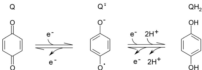
Fig. 1. Redox reactions of the quinone ring, Q—oxidized form, \text{Q}^{\cdot-} —charged, semiquinone radical, unstable, can be stabilized by interaction with proteins, \text{QH}_2 —stable, non-charged hydroquinone form.
