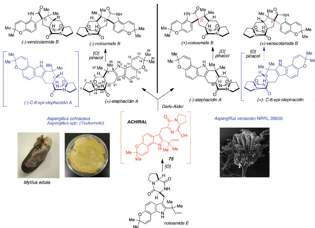
Scheme 22. Initial Biogenetic Hypothesis to Accommodate Enantio-divergent Production of Stephacidin A, Notoamide B, and Versicolamide B
