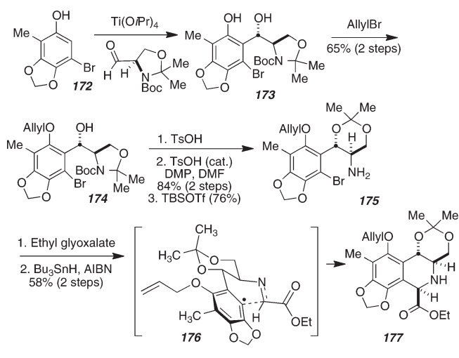
Scheme 41. Diastereoselective Tetrahydroisoquinoline Construction for Et-743
