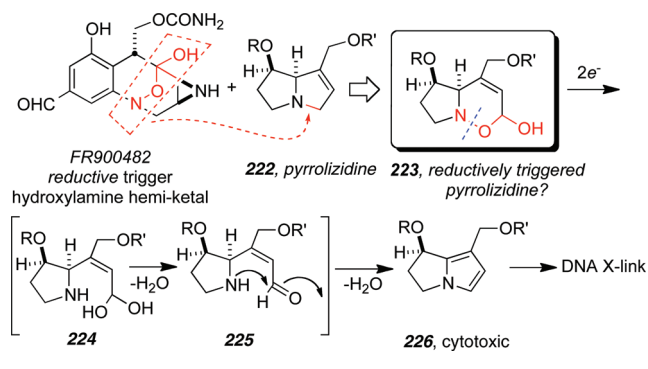
Scheme 53. Design of a “Chimeric” FR900482-Pyrrolizidine Alkaloid Hybrid
