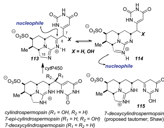
Figure 6. Biomechanistic queries on the cylindrospermopsins.
