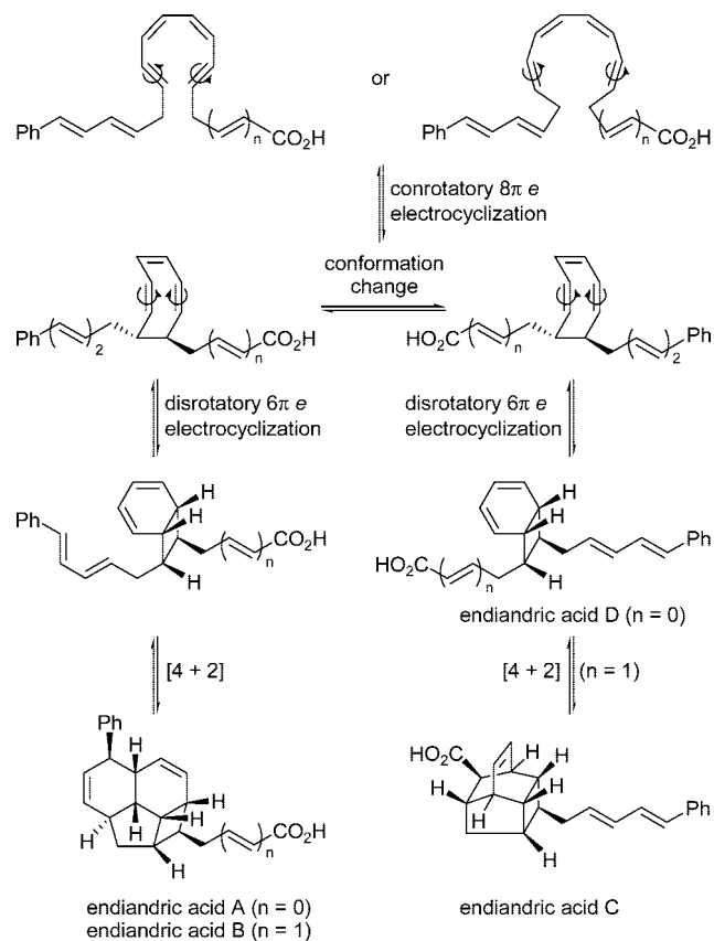
FIGURE 2. Black hypothesis for the biosynthesis of the endiandric acids (Black et al., 1980). 4
