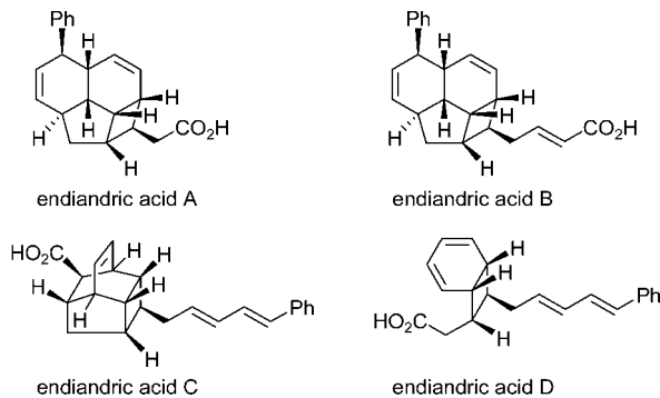
FIGURE 1. Molecular structures of endiandric acids A–D.
