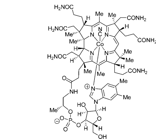
FIGURE 8. Molecular structure of vitamin B 12 .
