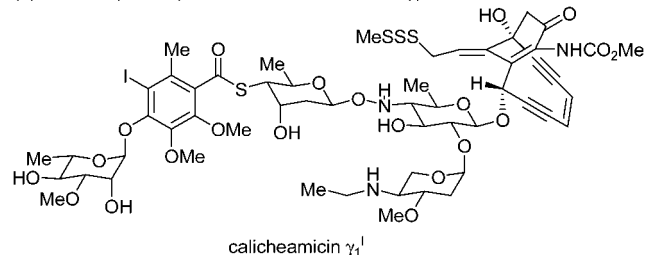
FIGURE 9. Originally proposed and revised molecular structure of calicheamicin \gamma_1^I .
