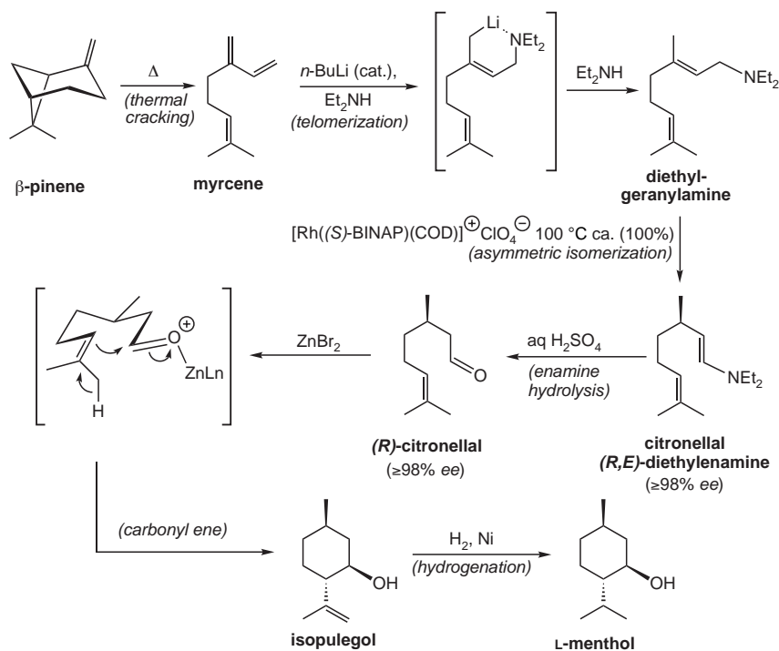
Figure 13. The Takasago process for the industrial production of L-menthol via catalytic asymmetric allylic amine \rightarrow enamine isomerization.
