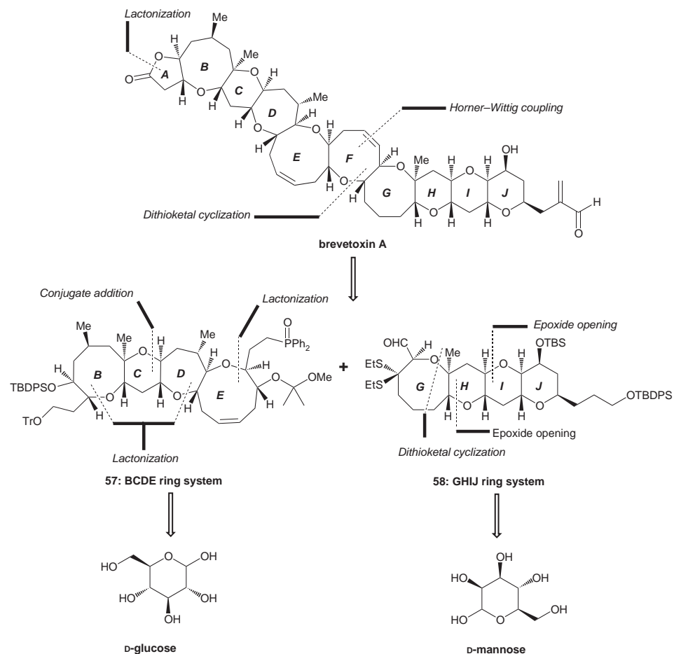
Figure 43. Retrosynthetic analysis and total synthesis of brevetoxin A (Nicolau, 1997).
