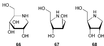
Fig. 15 Sugar-mimic alkaloids from the mulberry Morus australis . 272
