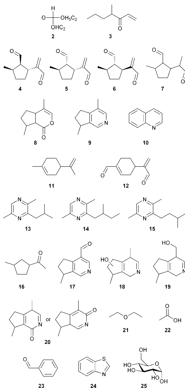
Fig. 5 Compounds from the defense glands of phasmids.
