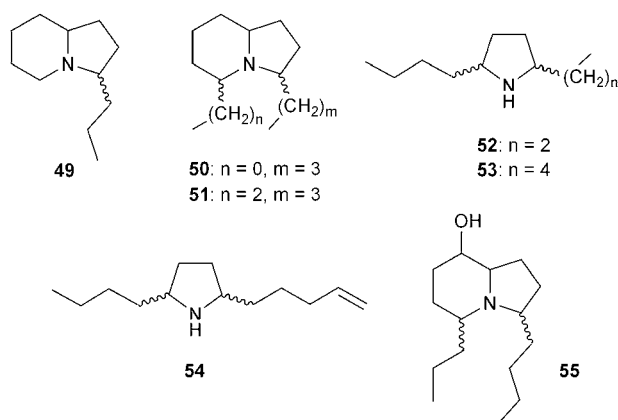
Fig. 8 Alkaloids from the Bornean ant Myrmecaria melanogaster . 178 Where the sidechain relative configurations are shown as ambiguous, either multiple stereoisomers were identified in the original report or no relative configuration was reported.
