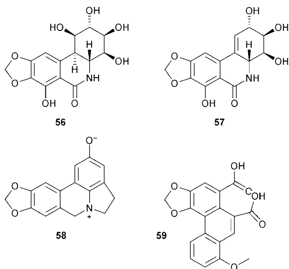
Fig. 9 Cytotoxic compounds from the Texas lubber grasshopper Brachystola magna and the butterfly Byasa polyeuctes termessa .
