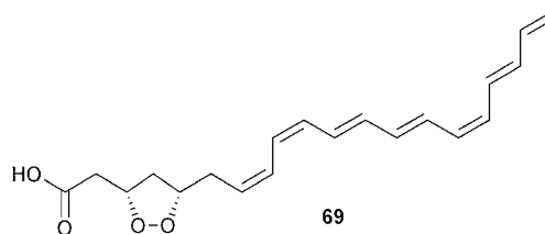
Fig. 16 Mycangimycin ( 69 ) from the bacterial species Streptomyces sp. SPB74, a mutually beneficial symbiont of the southern pine beetle Dendroctonus frontalis . 274
