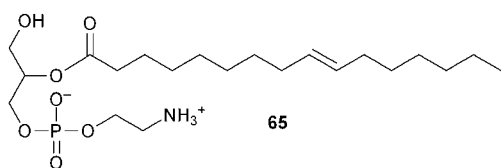
Fig. 14 1-Lysophosphatidylethanolamine (C16:1) ( 65 ), an antimicrobial lysophospholipid from the housefly Musca domestica . 246
