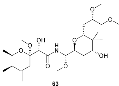
Fig. 12 Pederin ( 63 ), a defensive compound from the rove beetle Paederus fuscipes . 44,220,221
