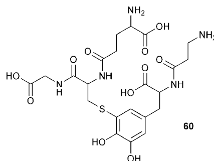
Fig. 10 5- S -GAD ( 60 ) from the flesh fly Sarcophaga preegrina . 159,216–218
