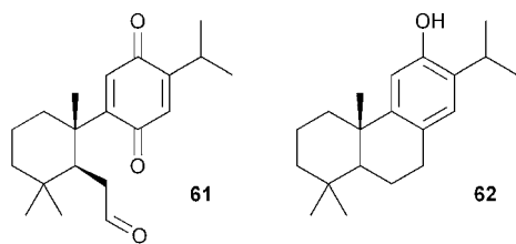
Fig. 11 Compounds from the nests of Vespa simillima ( 61 ) and from a likely source of its nest material, Cryptomeria japonica ( 62 ). 219
