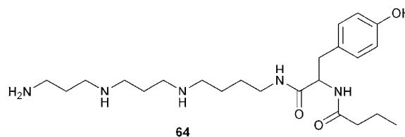
Fig. 13 Philanthotoxin ( 64 ), a neurotoxin from venom of the predatory digger wasp Philanthus triangulum . 224–227
