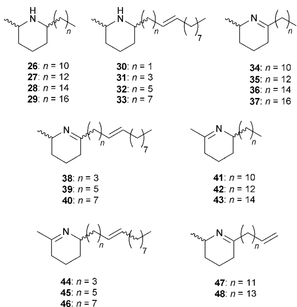
Fig. 7 Solenopsins, the major active substances from the venom of ants in the genus Solenopsis (such as S. invicta ). 174–177,280 Where the relative configurations are ambiguous in this figure, either multiple stereoisomers were identified in the original report or no relative configuration was reported.
