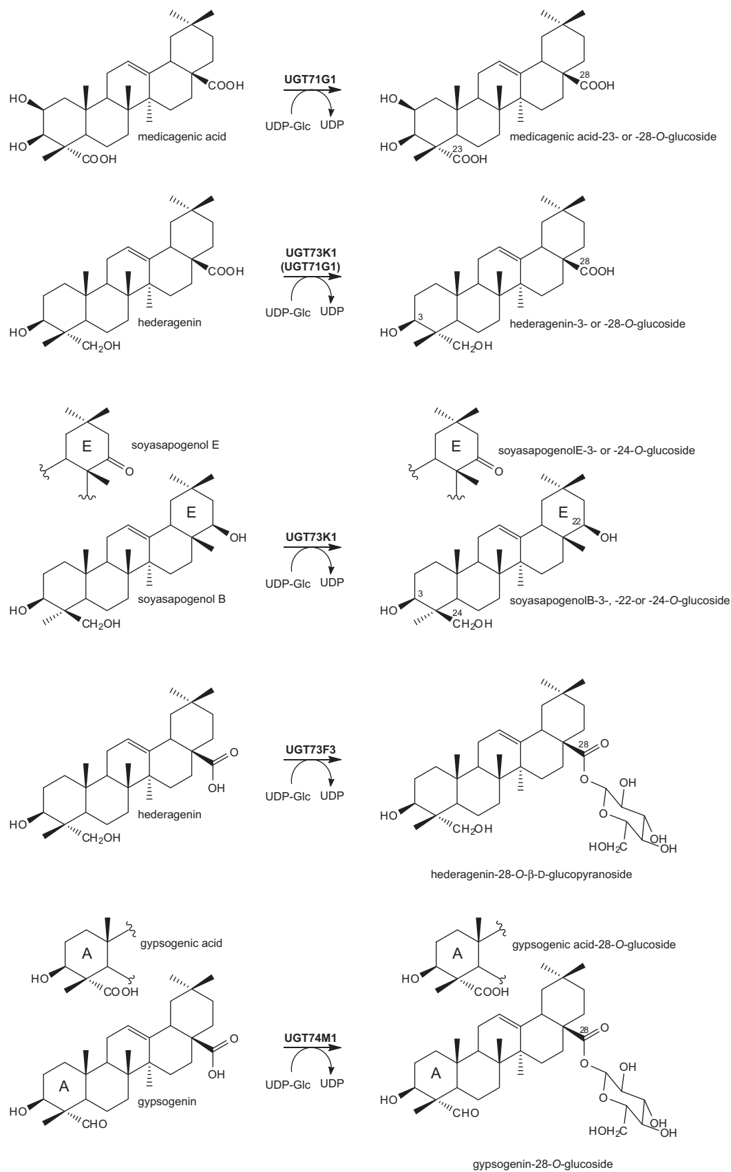
Fig. 10. Glycosylation of oleanane type saponins by UGTs in triterpenoid saponin biosynthesis. The position specificity of UGT71G1 and UGT73K1 has not been elucidated. Putative glycosylation positions suggested by the authors are indicated by numbering (biochemical activities are according to Achnine et al., 2005; Meesapyodsuk et al., 2007; Naoumkina et al., 2010).
