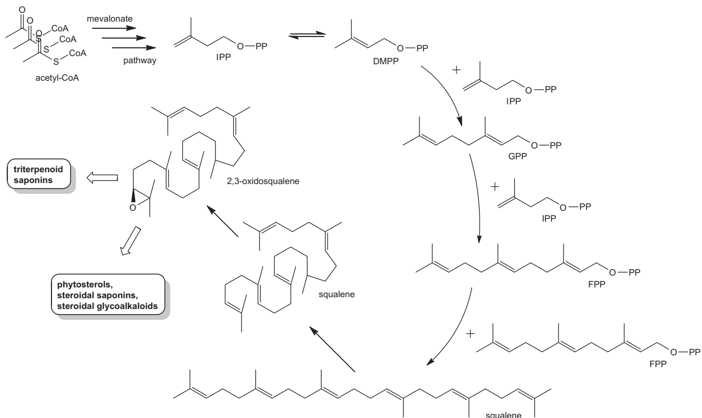
Fig. 6. Early steps in biosynthesis of phytosterols and triterpenoid saponins leading to the common precursor 2,3-oxidosqualene. IPP – Isopentenyl pyrophosphate, DMAPP – dimethylallyl pyrophosphate, GPP – geranyl pyrophosphate, FPP – farnesyl pyrophosphate.
